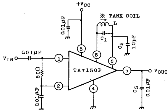
TEST CIRCUIT 1
